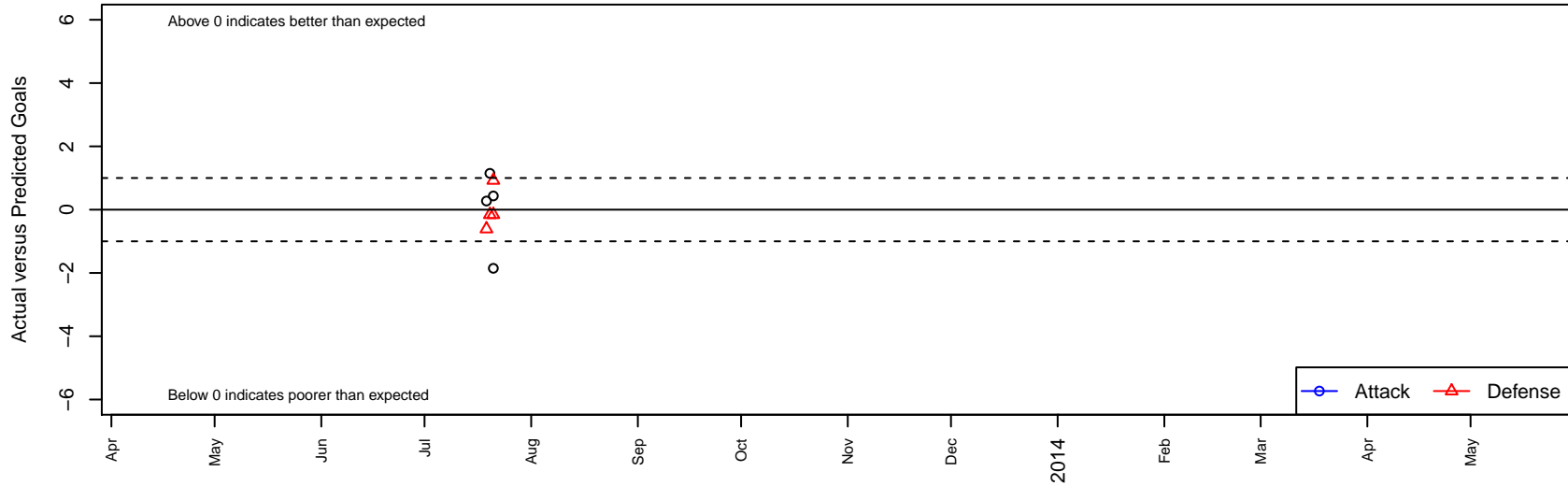
Santos – Unk B01 Dots are actual minus expected GF (blue circles) and GA (red triangles). Blue line is smoothed change in attack strength. Red is smoothed change in defense strength.
